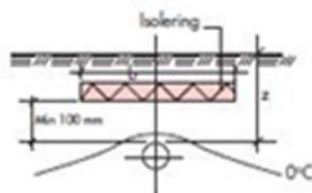
Figur 24. Horisontell isolering.
